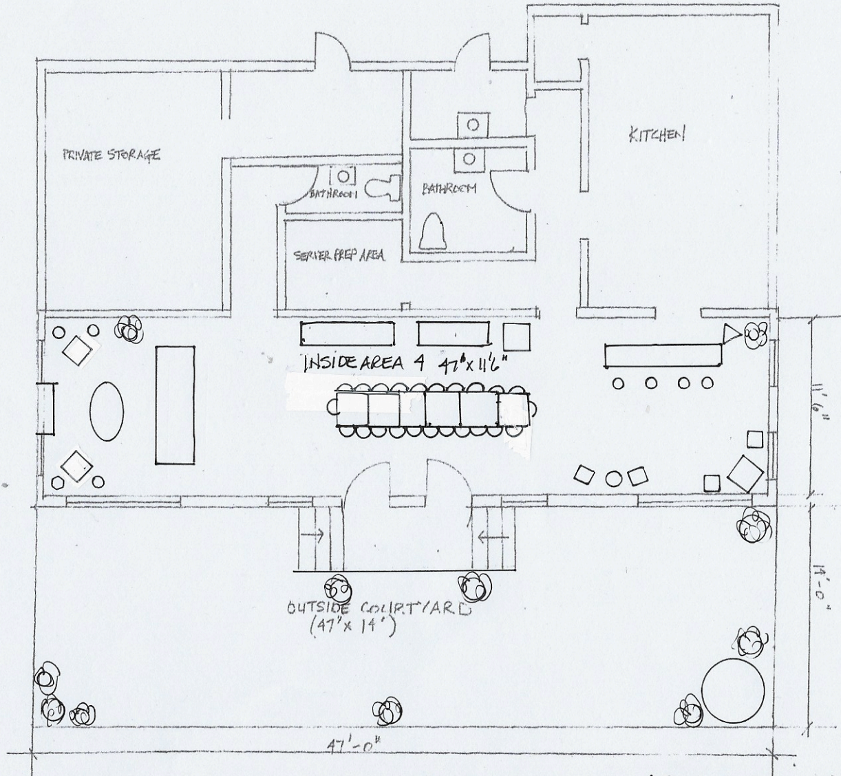
INSIDE FAMILY DINING - FLOOR PLAN
