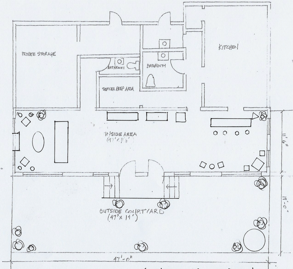
GENERAL FLOOR PLAN
